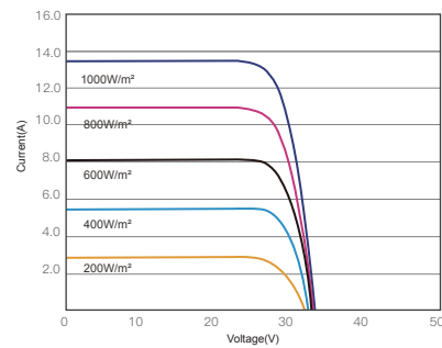
I-V CURVES OF PV MODULE(440W)
