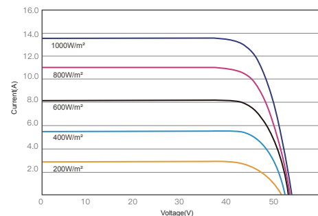
I-V CURVES OF PV MODULE(575W)
