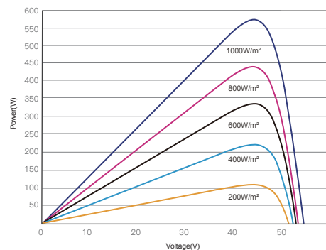
P-V CURVES OF PV MODULE(575W)
