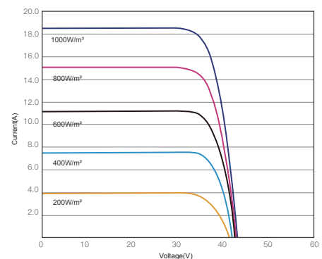
I-V CURVES OF PV MODULE(595W)
