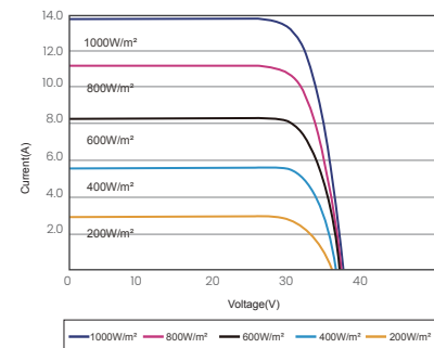
I-V CURVES OF PV MODULE(415W)
